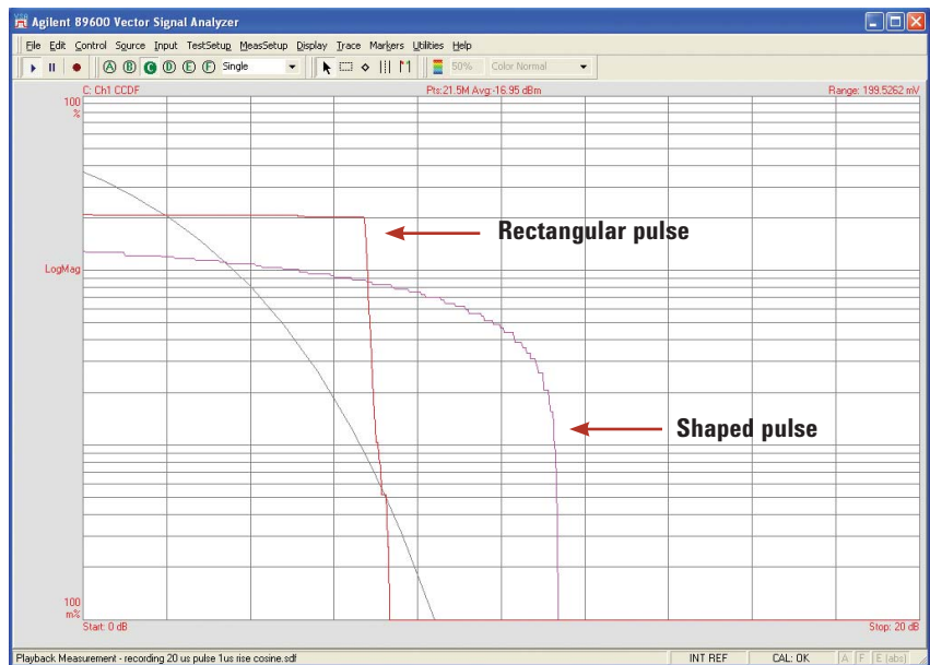
Figure 32. CCDF measurement of a square pulse radar signal compared to a raised-cosine-shaped pulse radar signal. A CCDF plot describes the power statistics of a signal by plotting the percentage of time (y axis) the signal spends at x dB above the average power (x axis).
