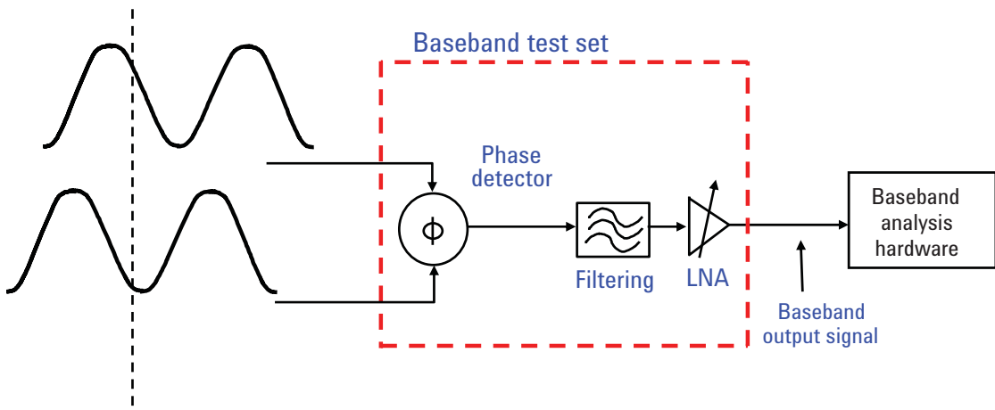
Figure 53. A basic block diagram of phase detector-based phase noise measurement. The measurement compares the test signal to a phase-locked reference signal with a phase detector. Variations in phase due to phase noise result in a voltage output that is then processed to determine the phase noise result.
