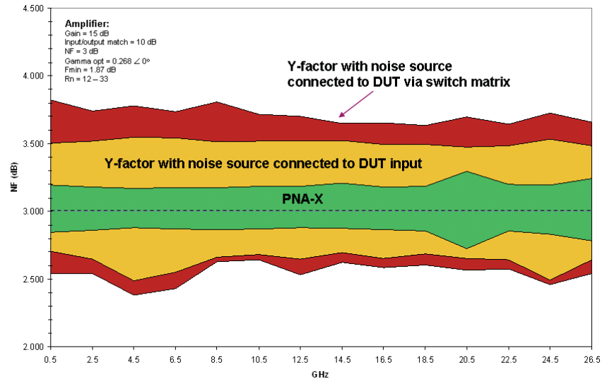
Figure 50. PNA-X-based noise figure solution provides the best measurement uncertainty due to its high sensitivity and ability to use vector error corrections to subtract errors due to effects such as impedance mismatch.
