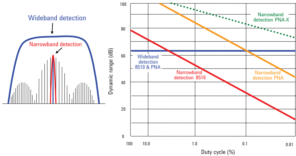
Figure 39. The effects of duty cycle on dynamic range are shown by comparing network analyzer wideband detection and narrowband detection modes
