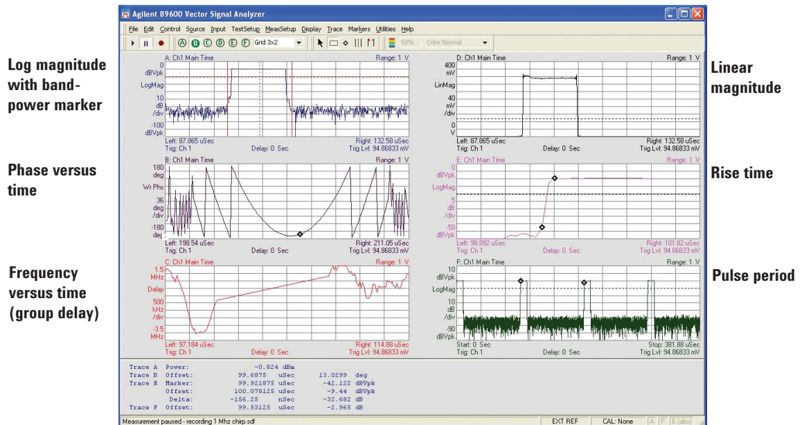
Figure 28. Time-domain measurements on chirp radar using a vector signal analyzer
