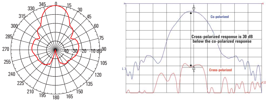
Figure 47. Examples of a far-field antenna pattern and a cross-polarization measurement. The gain can be measured and compared using different polarization orientations of the antenna.
