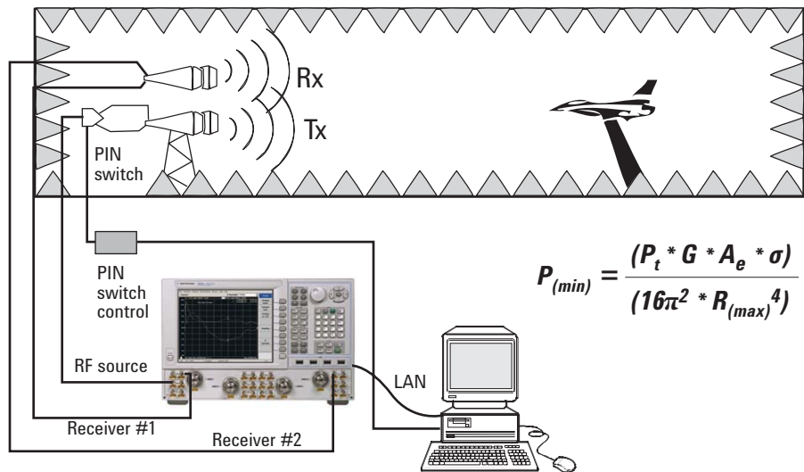
Figure 48. This example radar cross section measurement setup uses a network analyzer and an anechoic chamber.
