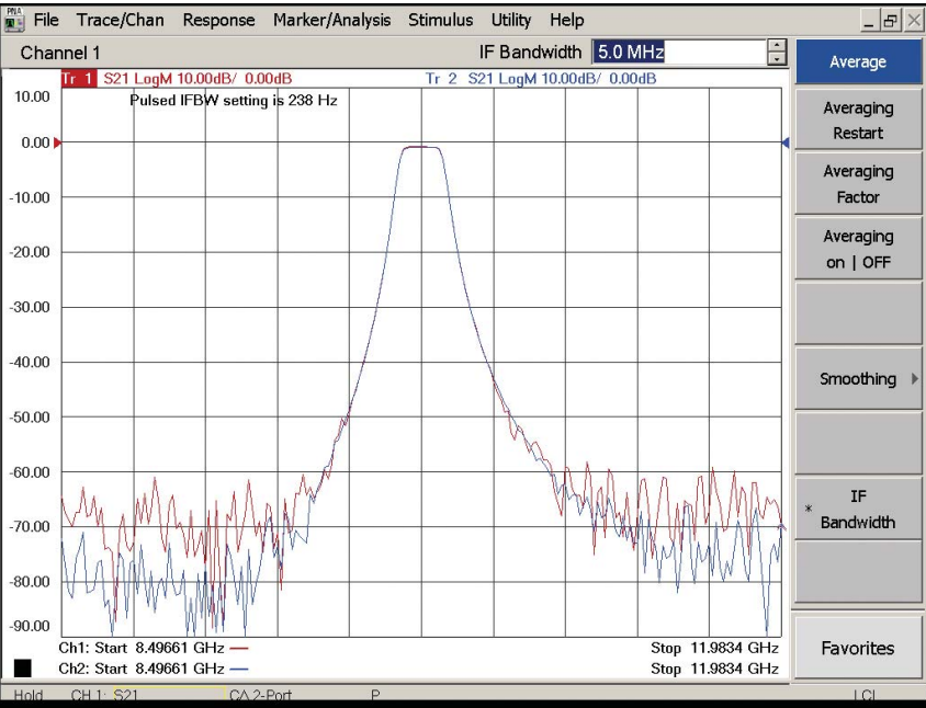
Figure 38. This display shows a comparison of a pulsed insertion loss filter measurement using the wideband mode versus the narrowband mode in the PNA-X network analyzer. In this example, the narrowband mode achieves the best dynamic range; however, which mode is best will depend on the duty cycle.
