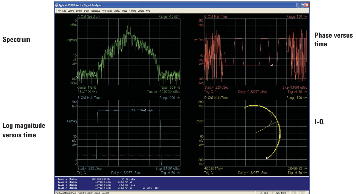
Figure 33. A vector signal analyzer has the ability to examine phase variations over time. This is a useful feature for examining a Barker coded pulse with code embedded in the phase transitions.
