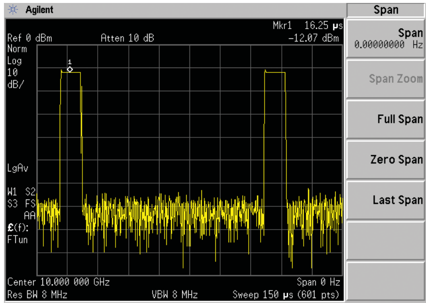
Figure 18. This example of zero-span mode gives a time-domain view of the envelope of the radar pulse. It is a convenient way to measure pulse characteristics when the bandwidth of the radar signal is much less than the RBW of the spectrum analyzer.
