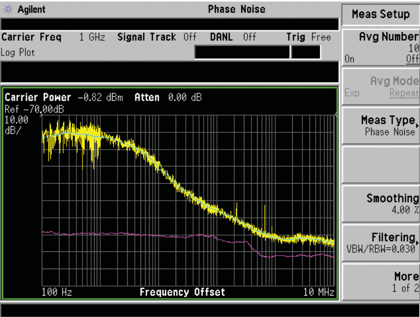
Figure 52. With the PSA spectrum analyzer phase noise measurement personality, results are displayed as a function of offset frequency from the carrier
