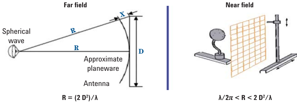
Figure 42. Antenna measurements can be made using either a far-field or near-field approach. Far-field testing is simpler and faster but requires a large area. Near-field testing requires sophisticated calculations and may take longer to perform, but requires less space.
