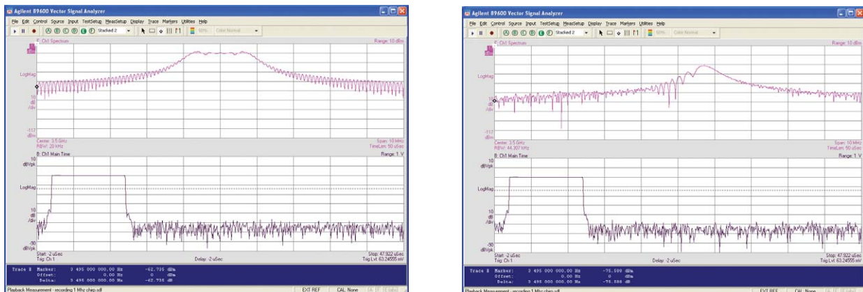
Figure 27. This compares a radar measurement made on a VSA using different windowing functions, uniform (left) and Gaussian (right). The Gaussian window distorts the spectrum because the pulse occurs near the start of the measurement time window. Because pulsed radar signals are self-windowing, the uniform window function should be used to ensure the best accuracy.
