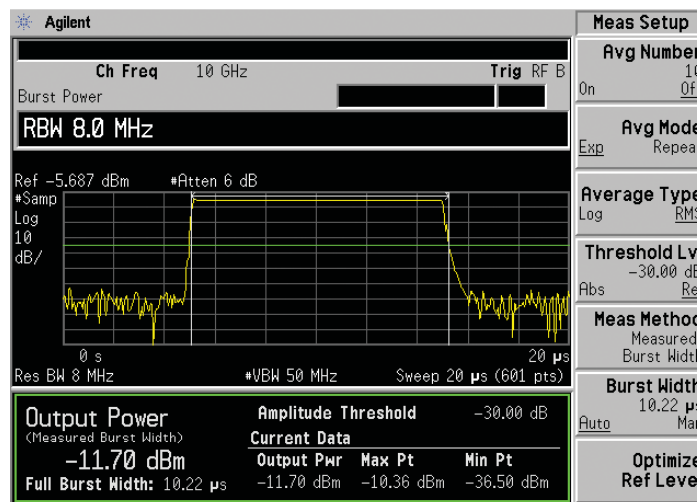
Figure 22. This is an example of burst-power measurement from the PSA spectrum analyzer. Burst power and pulse width are automatically measured in zero-span mode.
