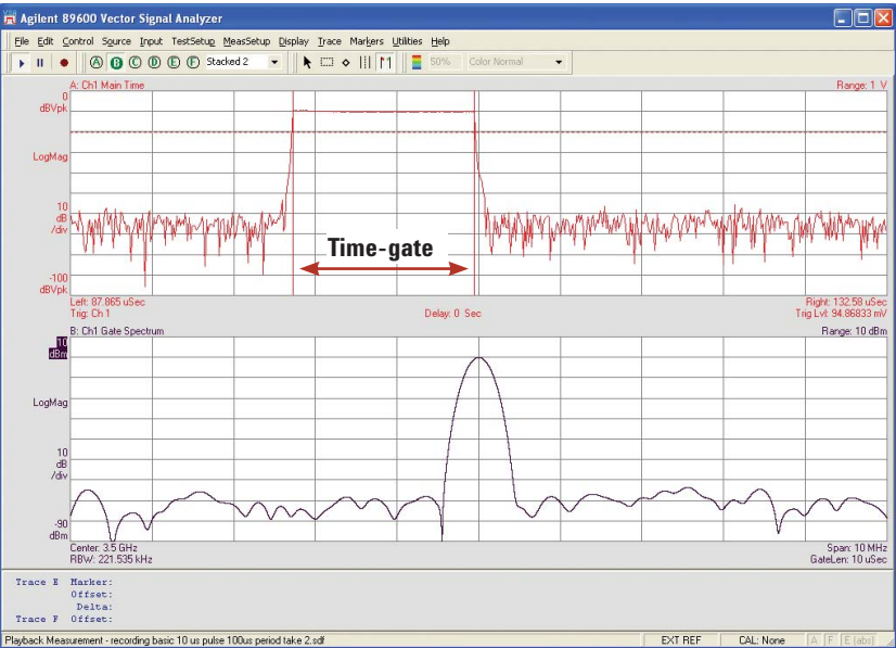
Figure 29. This is a time-gated measurement of simple RF pulse showing CW spectrum of signal when pulse is on
