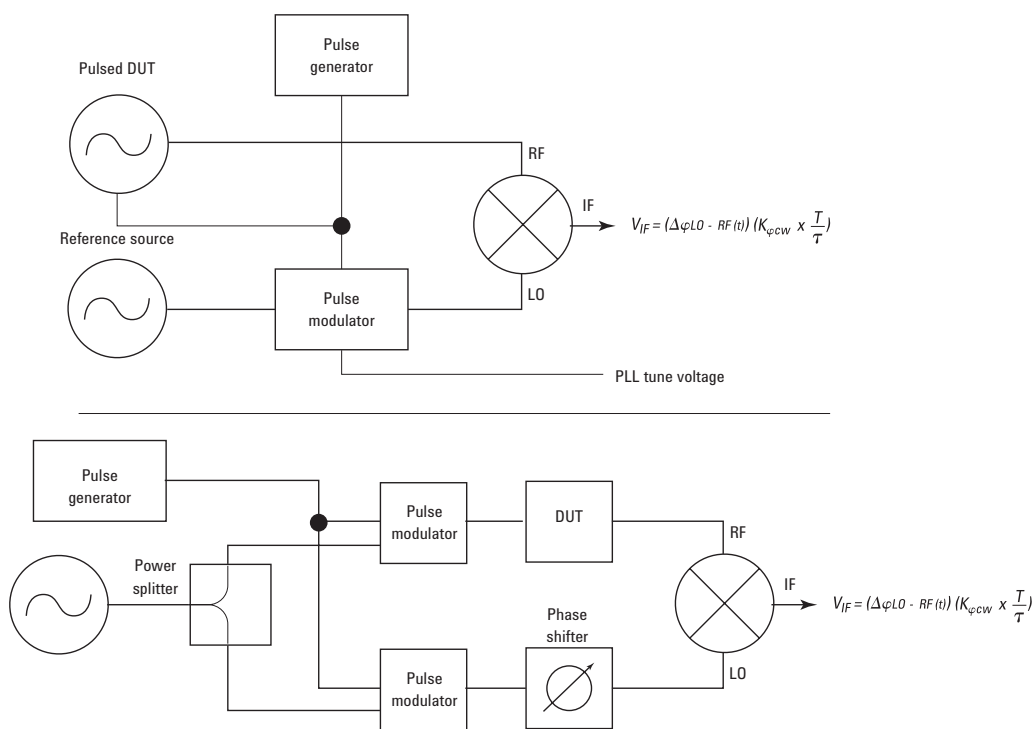
Figure 56. Test configuration for making absolute and residual pulsed phase noise measurements using the Agilent E5500 phase noise test system
