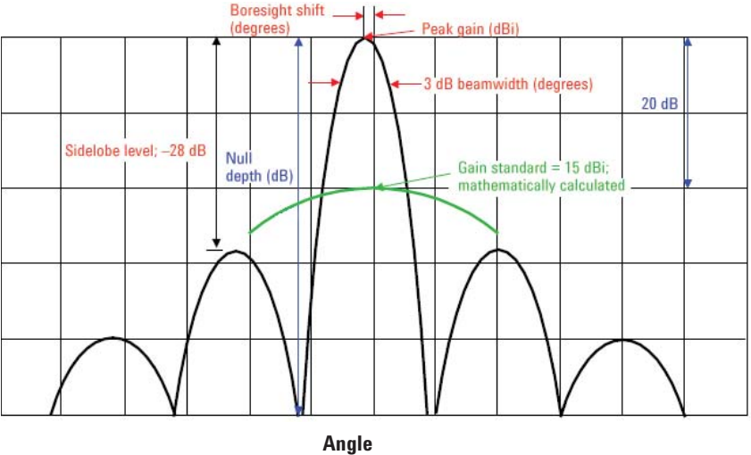
Figure 41. Many importance characteristics of the antenna can be determined from the antenna pattern.
