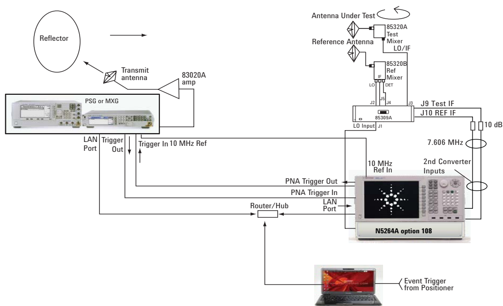
Figure 43. In this example of a far-field antenna test configuration, external mixers are used so that they can be placed close to the reference and test antenna. Directly inputting the IF signal into the PNA second mixing stage also improves measurement sensitivity.
