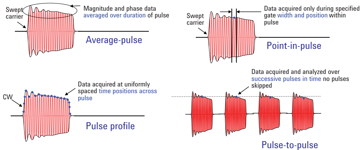
Figure 40. For radar applications, the Agilent PNA has four different pulse-sampling options
