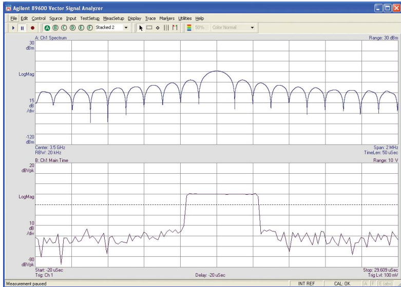
Figure 25. A vector signal analyzer has the ability to provide spectrum analysis of a single pulse.
