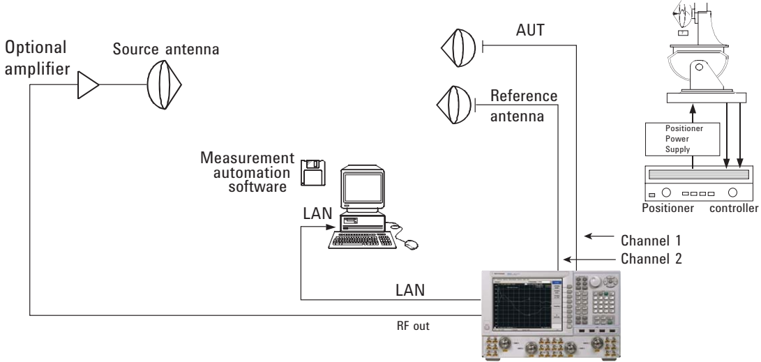
Figure 44. This example of a simple test configuration with a network analyzer is used for smaller far-field test setups, but may not be possible for large ranges due to cable losses.
