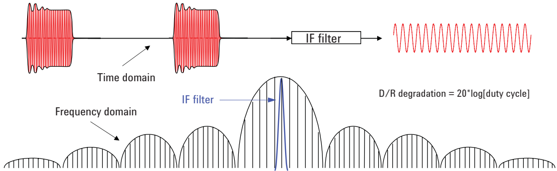
Figure 37. The narrowband detection mode (asynchronous detection mode) of a network analyzer uses a narrow filter to extract only the central spectral component. The narrowband mode has no pulse width limitations.
