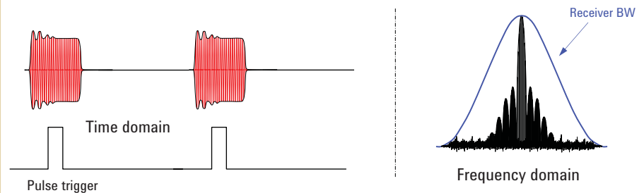
Figure 36. Wideband detection mode (synchronous detection mode) of a network analyzer requires the majority of the pulse power be contained within the receive bandwidth of the network analyzer. Wideband mode may have the best dynamic range for signals with low duty cycle but will be limited in measurable pulse widths due to bandwidth constraints.
