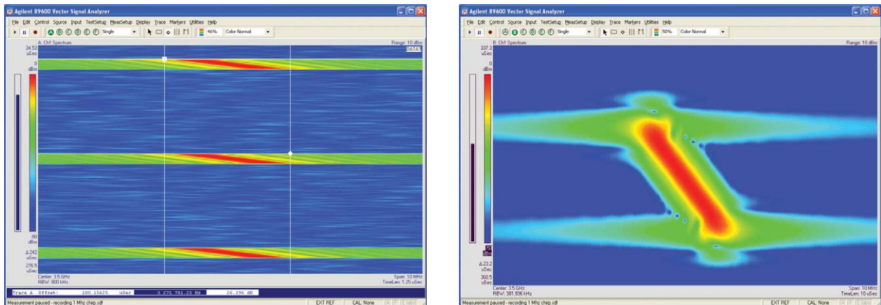
Figure 31. Spectrogram showing chirped radar signal. The left view shows the spectrogram of three consecutive pulses. The right view shows detailed view of a single pulse.
