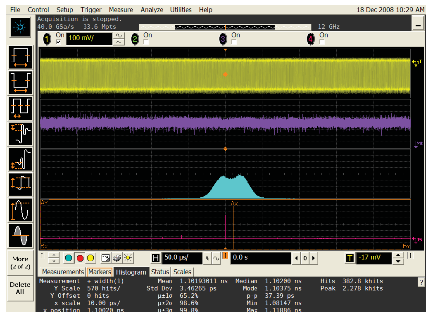
Figure 34. The built-in capabilities of the DS090000 series make it possible to acquire a chirped radar pulse with a bimodal PRI and then display a histogram of thousands of pulses.
