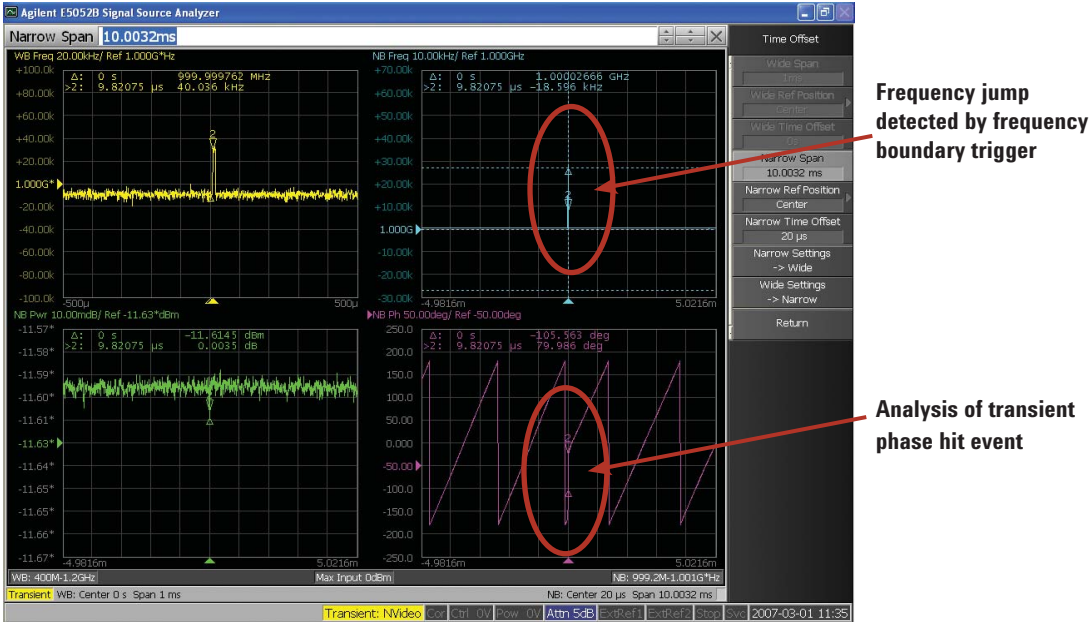
Figure 55. The SSA includes time-domain analysis and advanced trigger functions useful for examining transient events. In this screen, the analyzer is able to use its frequency-boundary trigger to capture and analyze a phase hit.
