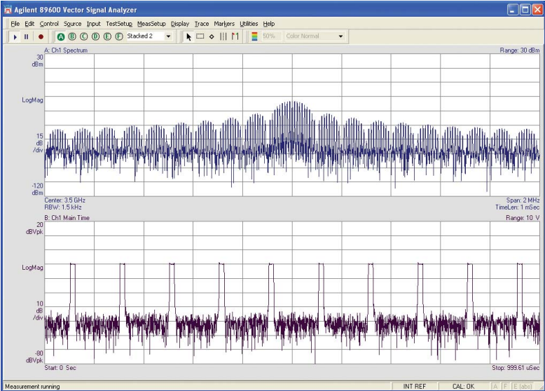
Figure 24. Vector signal analyzer measurement of radar pulse showing spectrum and time domain view
