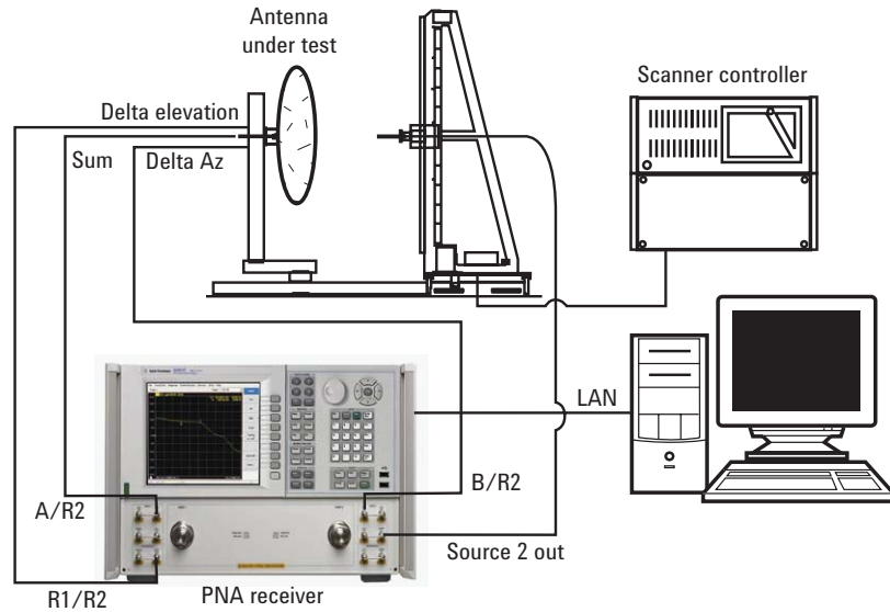
Figure 46. This is an example of a near-field antenna test configuration. Far-field antenna pattern results are extrapolated from the near-field measurements using transformational analysis.
