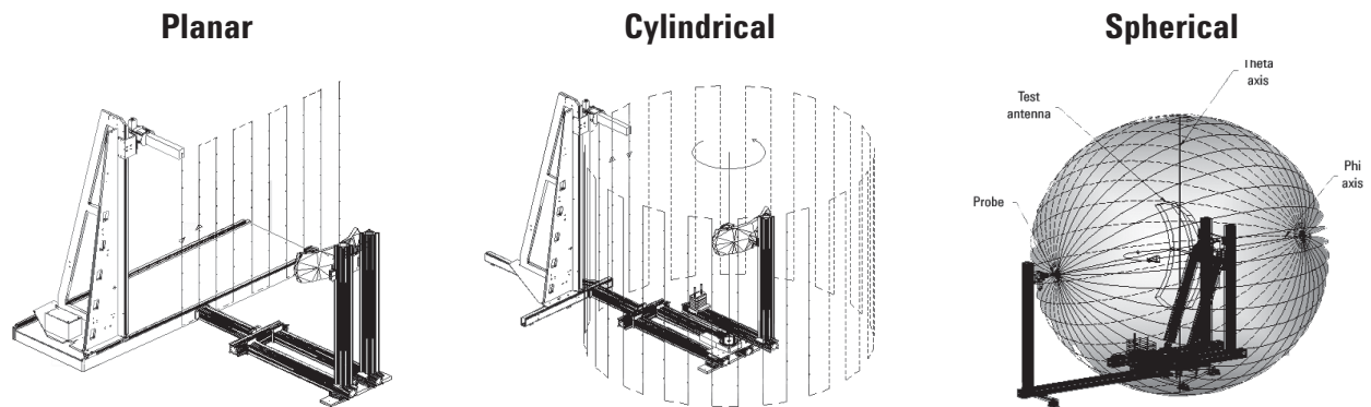
Figure 45. A near-field test uses different scan patterns depending on the type and purpose of the antenna.
