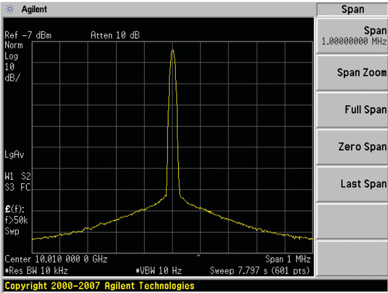
Figure 51. Phase noise results in sidebands that spread power into adjacent frequencies reducing the signal-to-noise ratio
