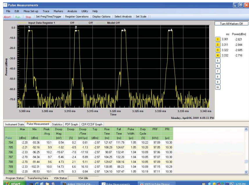
Figure 23. Running on a scope or signal analyzer, the N9051A software provides analysis of pulse parameters. This trace shows the results of zooming in and analyzing pulse-to-pulse amplitude variations with markers. It also shows results from automatic analysis of pulse metrics over 950 consecutive pulses.
