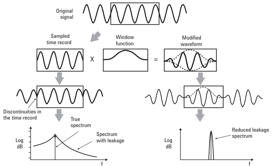
Figure 26. FFT analysis done in a spectrum analyzer or vector signal analyzer assumes a repeating signal. To minimize effects of discontinuities in the signal, a windowing function is used.
